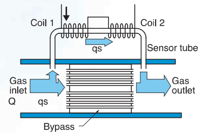
Basic design of the sensor
