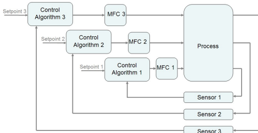
Figure 5 – Schematic illustrating multi-zone feedback control principal
