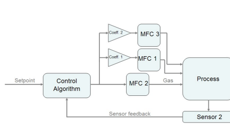
Figure 6 – Schematic illustrating master/slave control principal.
